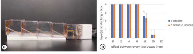
Figure 18: Effect of the offsets between boxes on box stacking: (a) experimental apparatus ( x = 4mm ) and (b) experimental results.
